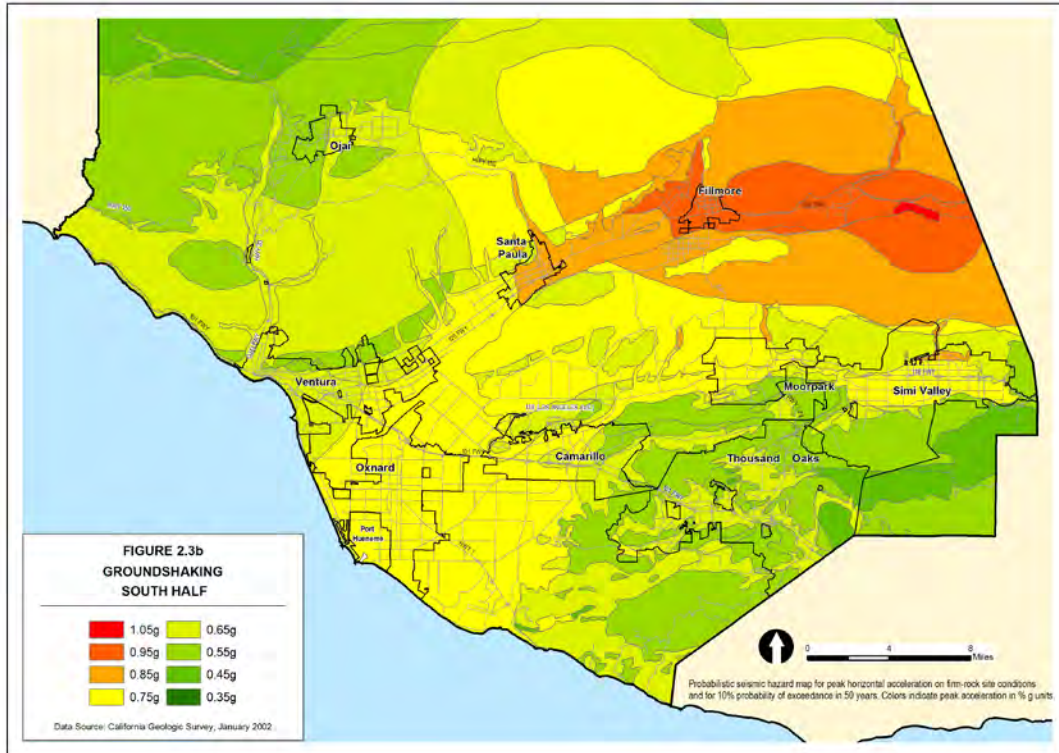
Figure 2.3b Ground Shaking Map - South Half
