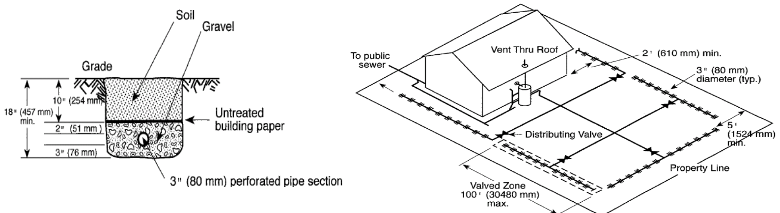
FIGURE 16-5 Gray Water System Typical Irrigation Layout.
